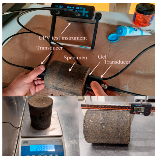
Figure 2. UPV testing.
