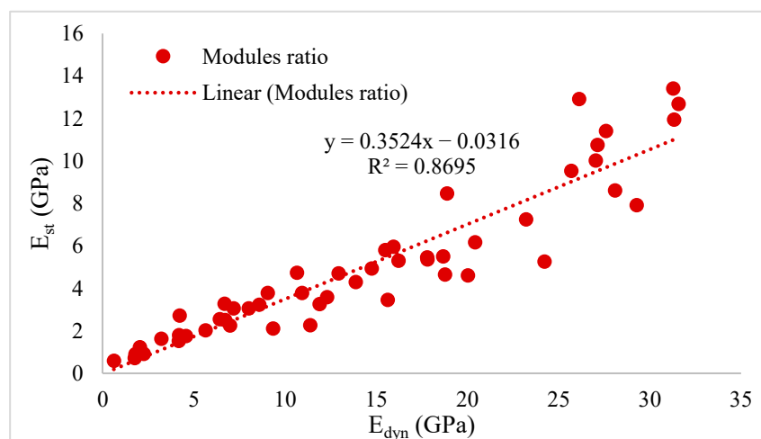
Figure 5. E_{dyn} and E_{st} relationship.
