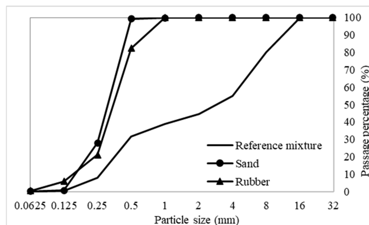
Figure 1. Granulometric composition.
