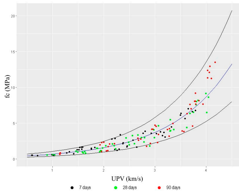
Figure 8. Mean predictions (blue line) and 2.5–97.5%-prediction-interval boundaries.
