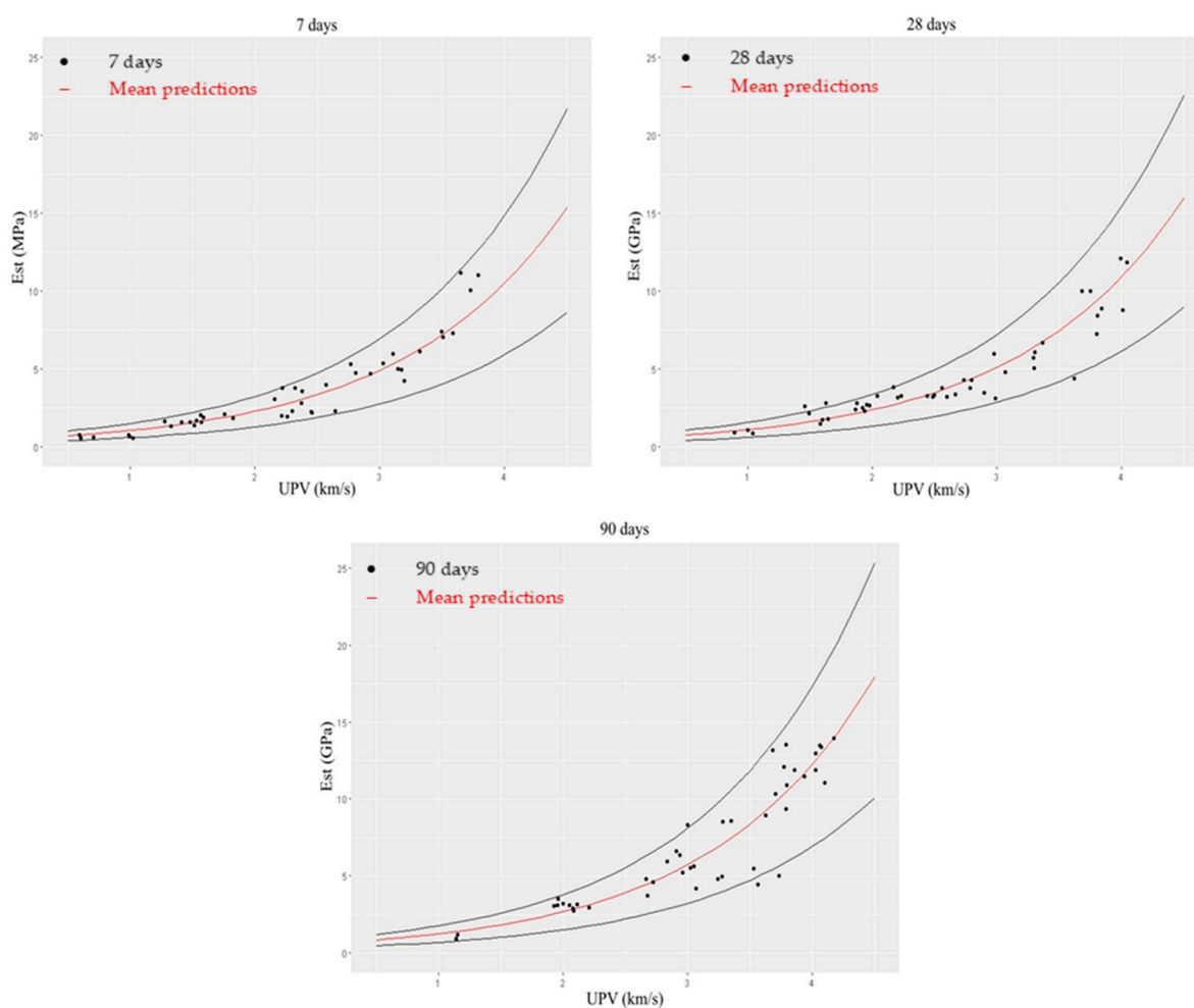
Figure 10. Mean predictions (red line) for E_{st} and 2.5–97.5%-prediction-interval boundaries.
