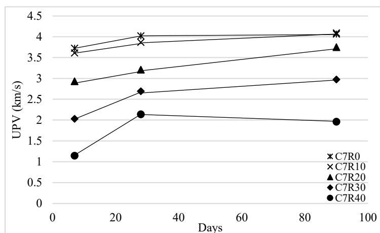
Figure 4. UPV development over time.
