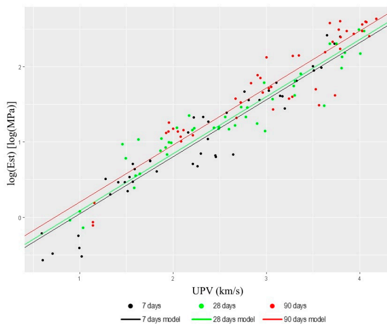
Figure 9. UPV- E_{st} relationship.
