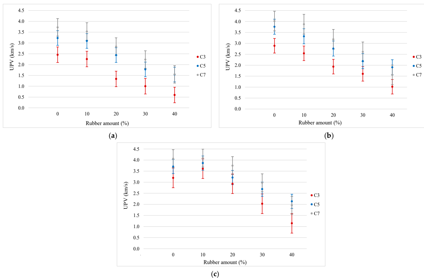
Figure 6. Impact of cement and rubber on UPV for curing periods of (a) 7 days, (b) 28 days and (c) 90 days.
