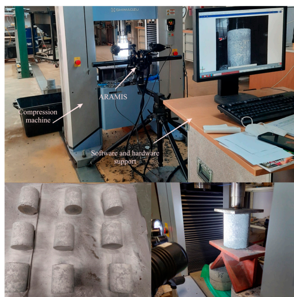
Figure 3. The f_c and E_{st} testing.
