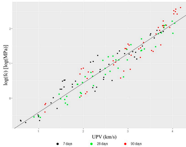
Figure 7. UPV- \ln(f_c) relationship.
