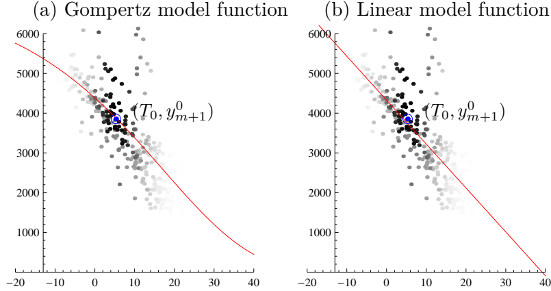
Figure 7: Data points and Gompertz and linear model function
