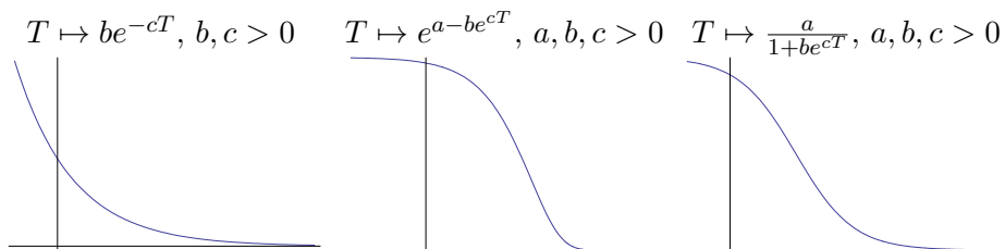
Figure 6: Exponential, Gompertz and logistic model function
