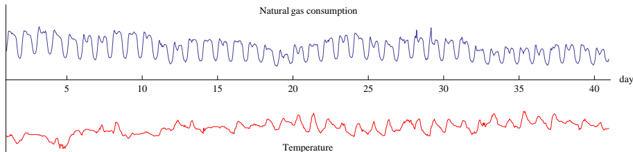
Figure 1: Air temperature and natural gas consumption in hourly intervals in the city of Osijek in the first 40 days in 2008
