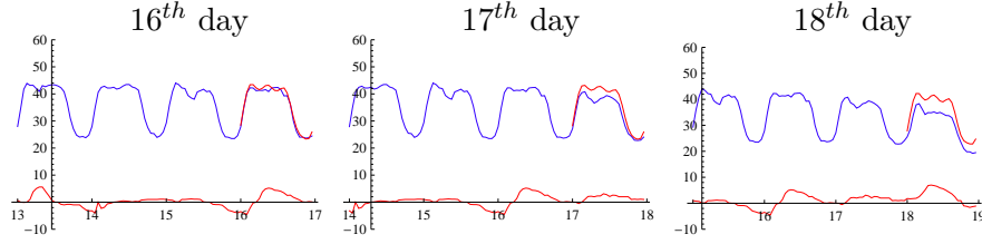
Figure 2: Forecast on the basis of linear – trigonometric model function
