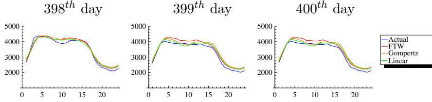
Figure 9: Comparison of actual daily natural gas consumption for three selected days (blue) and estimation obtained by applying the FTW-point (red), Gompertz model (orange) and linear model (green)
