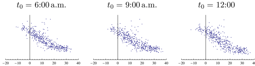
Figure 3: Dependence of natural gas consumption on temperature in Osijek at t_0 = 6:00 a.m., 9:00 a.m., 12:00
